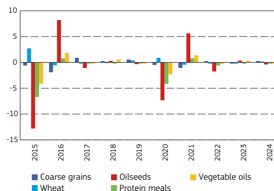
Graph 2.25 ENSO events – impact on world prices (%)
