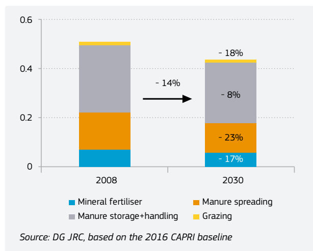
Graph 7.3 Projected ammonia emissions change by sources in Germany (million t of \text{NH}_3 )
