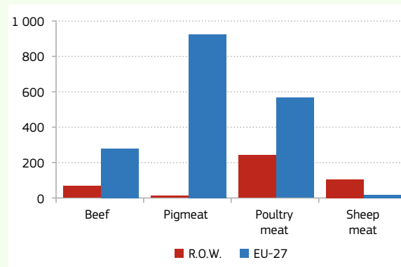
Graph 4.20 UK imports by meat type (average 2014–2016, 1 000 t)
