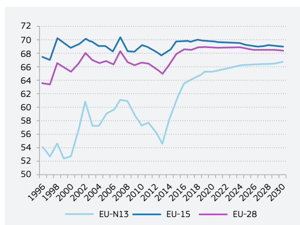
Graph 4.2 EU total meat consumption (kg per capita, retail weight)
