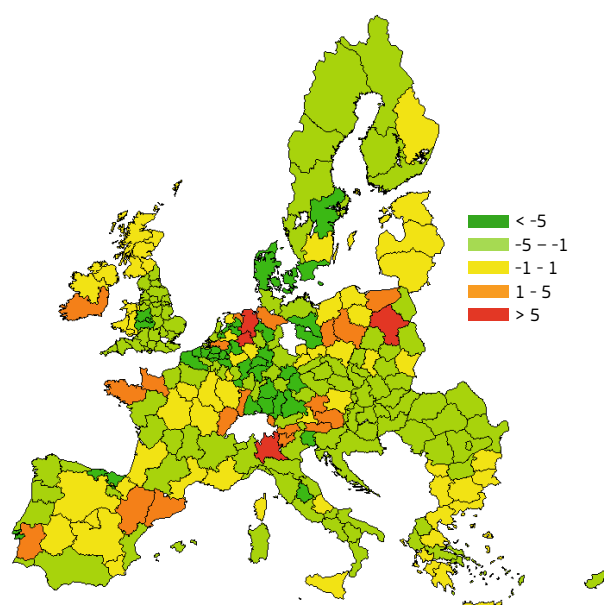
Map 7.3 Ammonia emissions change 2030-2008 (kg NH 3 /UAA ha)
