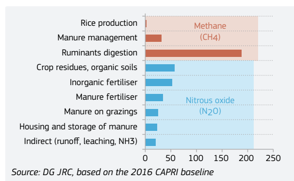
Graph 7.1 non-CO 2 GHG gas emissions sources in the EU-28 in 2030 (million t CO 2 equivalent) 67
