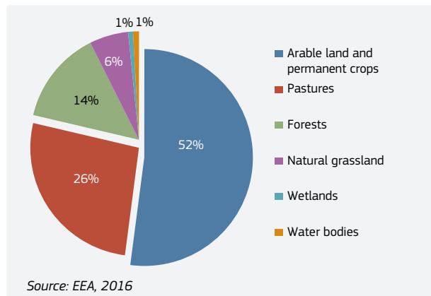
Graph 2.2 Contribution of land categories to uptake by urbanisation and other artificial land development (2006-2012)
